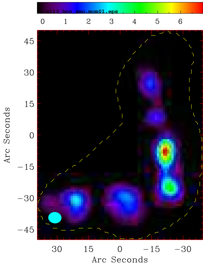
Intensity [JY/BEAM.KM/S]
