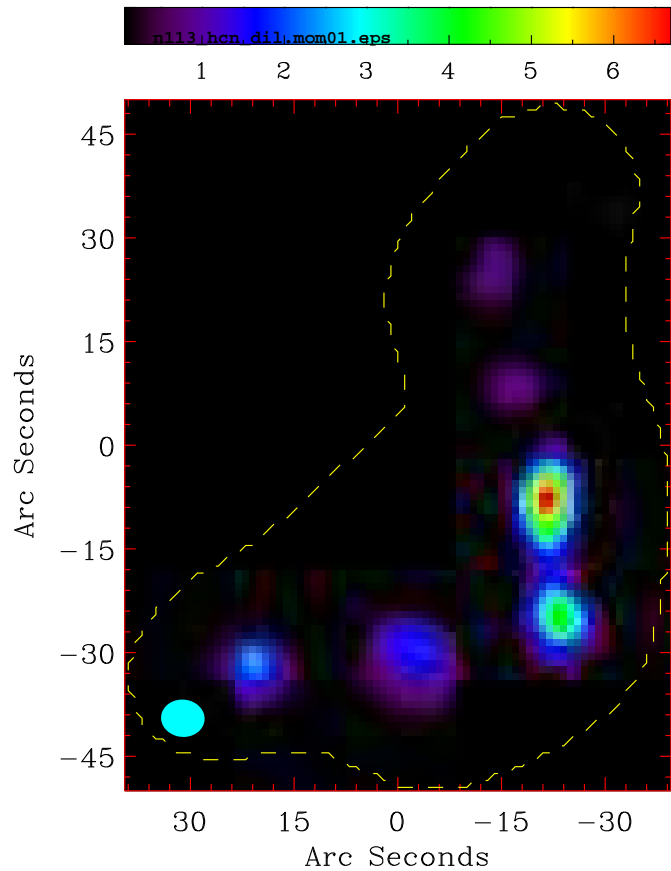
Intensity [JY/BEAM.KM/S]
